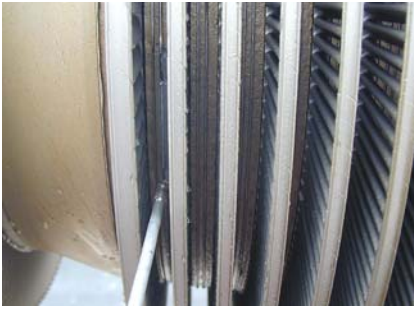
Turbine cleaning
